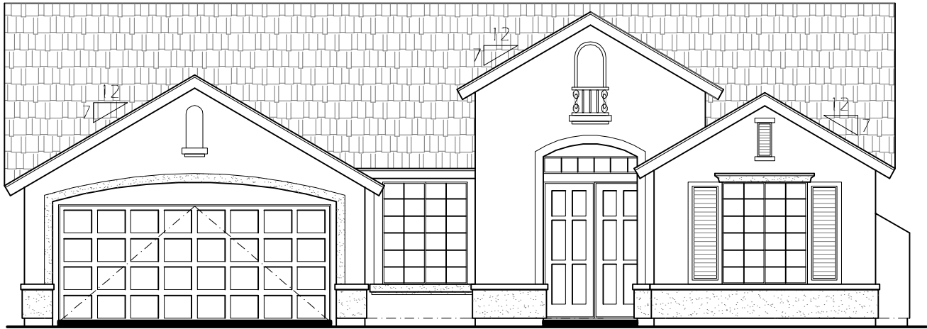
"A" ELEVATION - PLAN 2138 2-CAR (w/ 5:12 GABLE MAIN ROOF)
